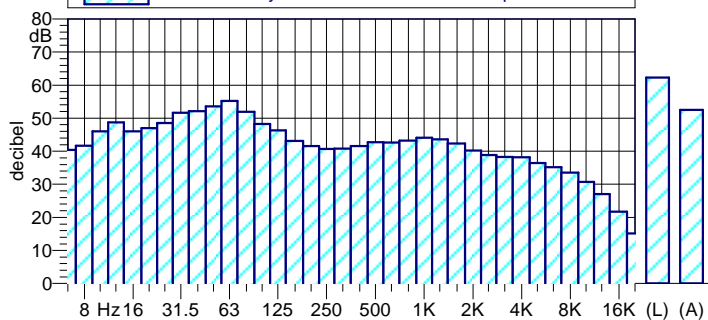
B) BORGIO By Time+SLM 11 - CH1 - Leq - Lineare
