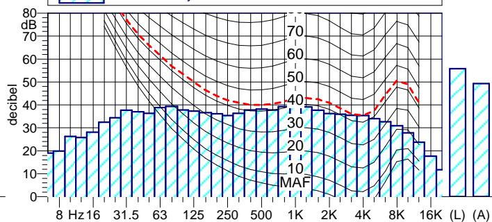
C) BORGIO By Time+SLM 11 - CH1 - Min - Lineare
